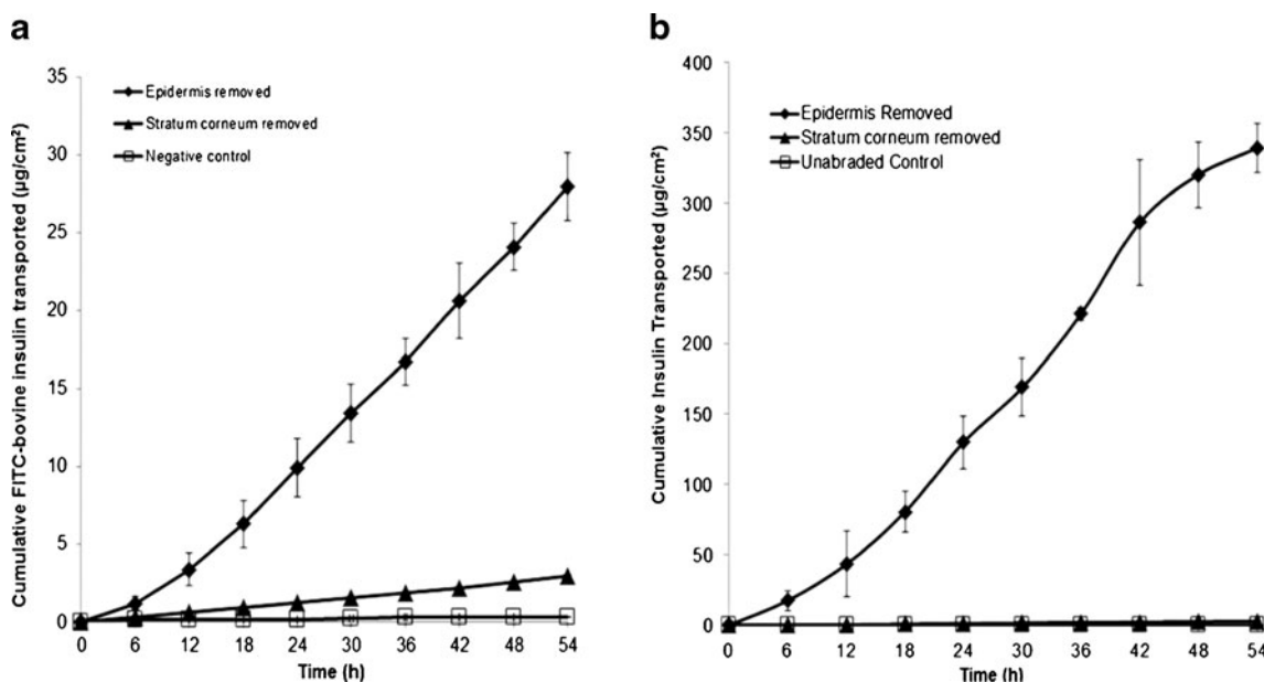
Fig. 7 The cumulative permeation of insulin across split-thickness human skin after tissue removal by microdermabrasion through a mask: unabraded skin (□), skin with stratum corneum removed by microdermabrasion at -30 kPa for 20 s (▲) and skin with full epidermis removed by microdermabrasion at -50 kPa for 60 s (◆). (a) Insulin delivery was determined by spectrofluorimetry based on permeation of FITC-labeled bovine insulin. (b) Insulin delivery was determined by ELISA based on permeation of recombinant human insulin (U-500 Humulin). Average \pm SD, n=3 . Permeation of insulin in (b) is greater than in (a) because the human insulin was provided at a higher concentration than the bovine insulin in the donor solution (see Materials and Methods).
