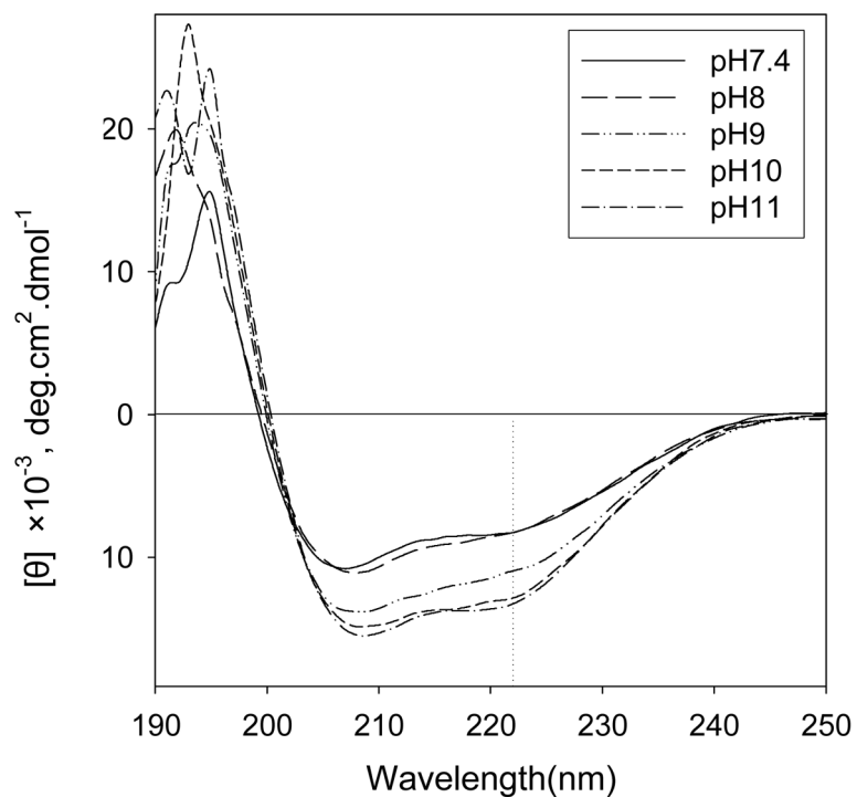
Figure 4. Circular dichroism spectra of magainin as a function of pH. Magainin was dissolved in 50 % ethanol at various pH values.
