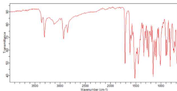
Figure 3: FTIR spectrum of Glibenclamide with Cinnamon Chloroform Extract.
