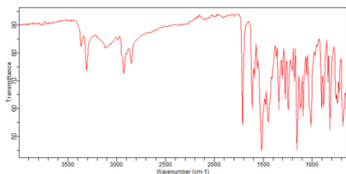
Figure 5: FTIR spectrum of Glibenclamide with Cinnamon Methanolic Extract.
