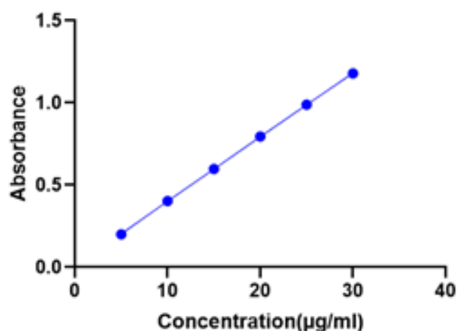
Figure 1: Calibration curve of Glibenclamide. 15
