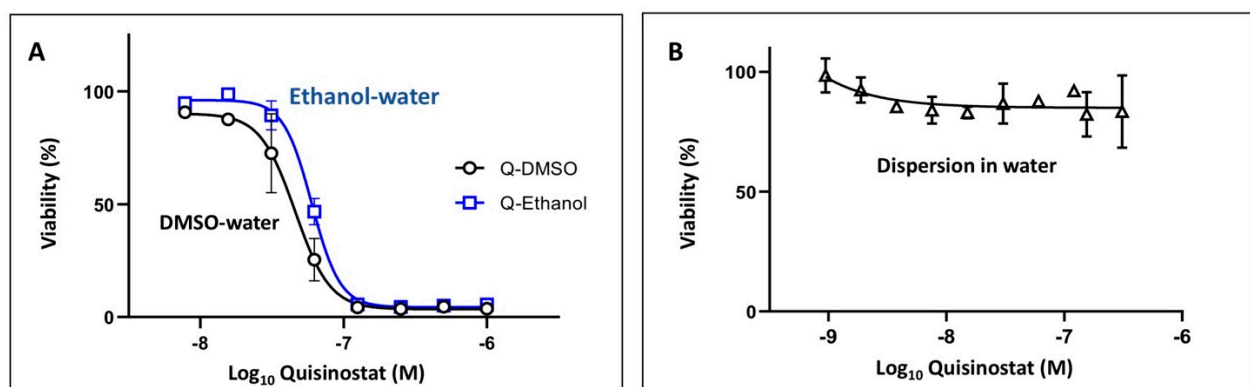
Figure A3. Representative dose–cell viability curves for quisinostat (A) dissolved in DMSO–water or ethanol–water mixtures and (B) dispersed in water (WM115 human melanoma cell line; 72 h, n = 3 ; points represent the mean values with errors indicating standard deviation).
